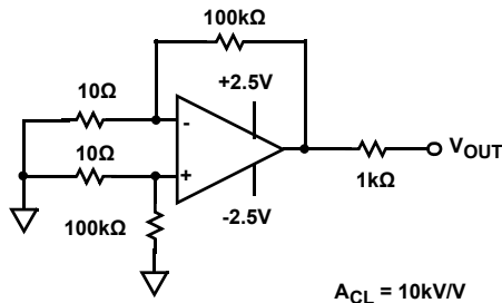
FIGURE 39. LONG TERM DRIFT TEST CIRCUIT
