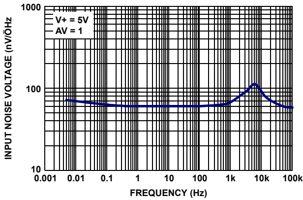
FIGURE 42. CHARACTERIZED INPUT NOISE VOLTAGE DENSITY vs FREQUENCY
